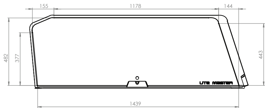
SIDE VIEW DOORS DOWN
