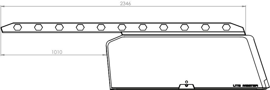
SIDE VIEW CANTILEVER ROOF RACK
